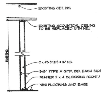
PARTITION SECTION (TYP.) SCALE: 1/2"=1'-0"
