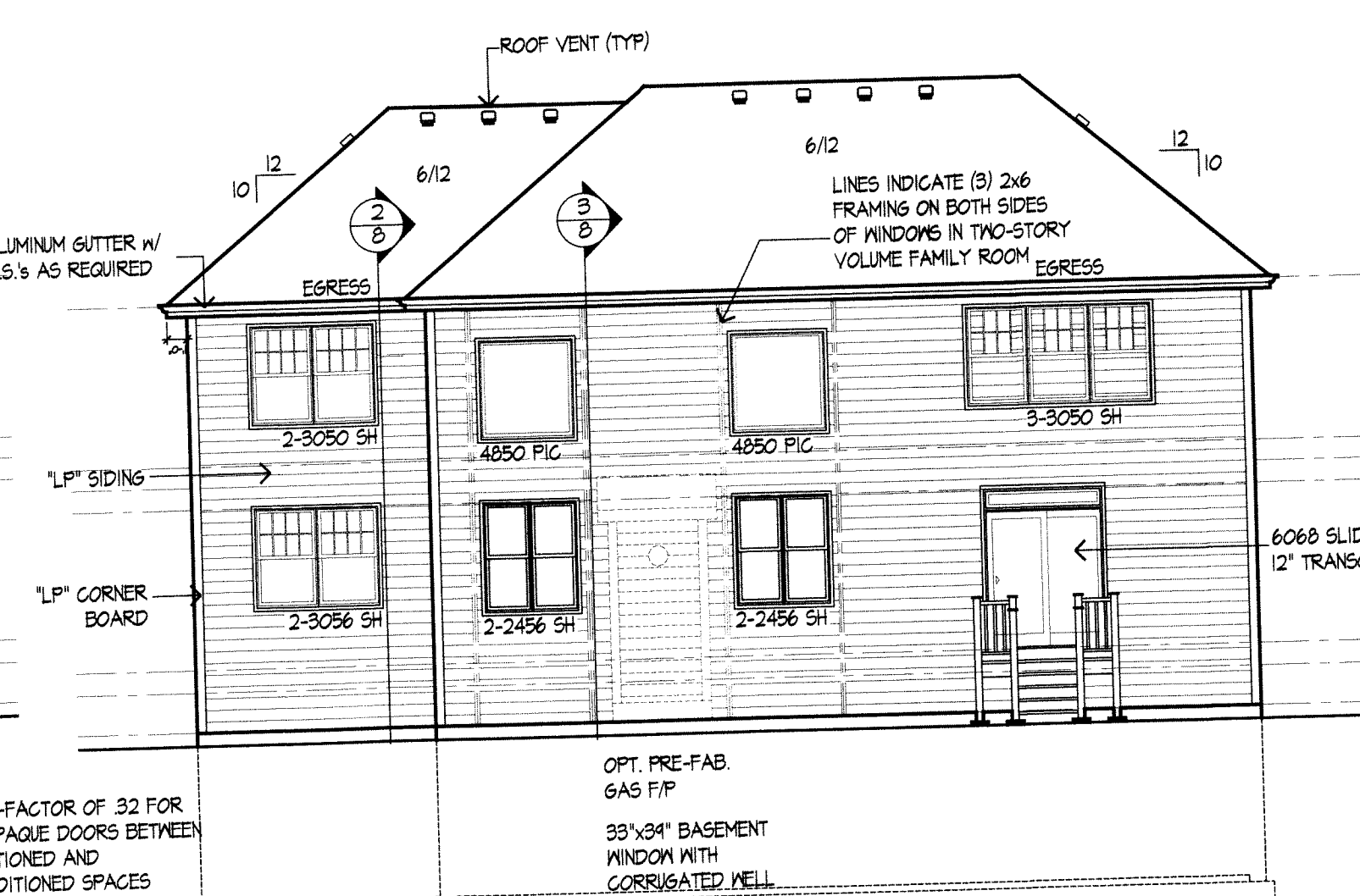
REAR ELEVATION
