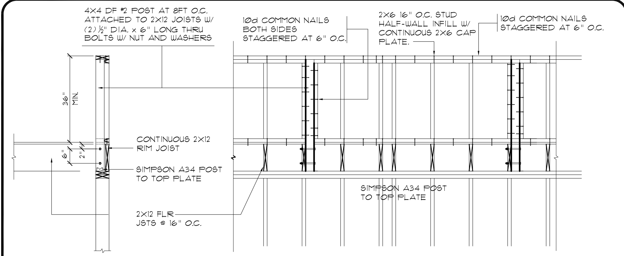
1 SECTION - HALF WALL FRAMING
