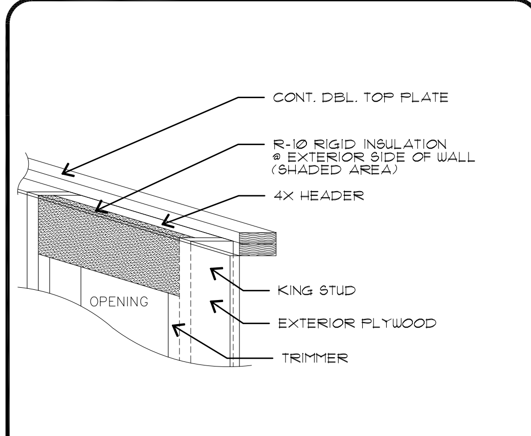
2 HEADER/INSULATION DETAIL
