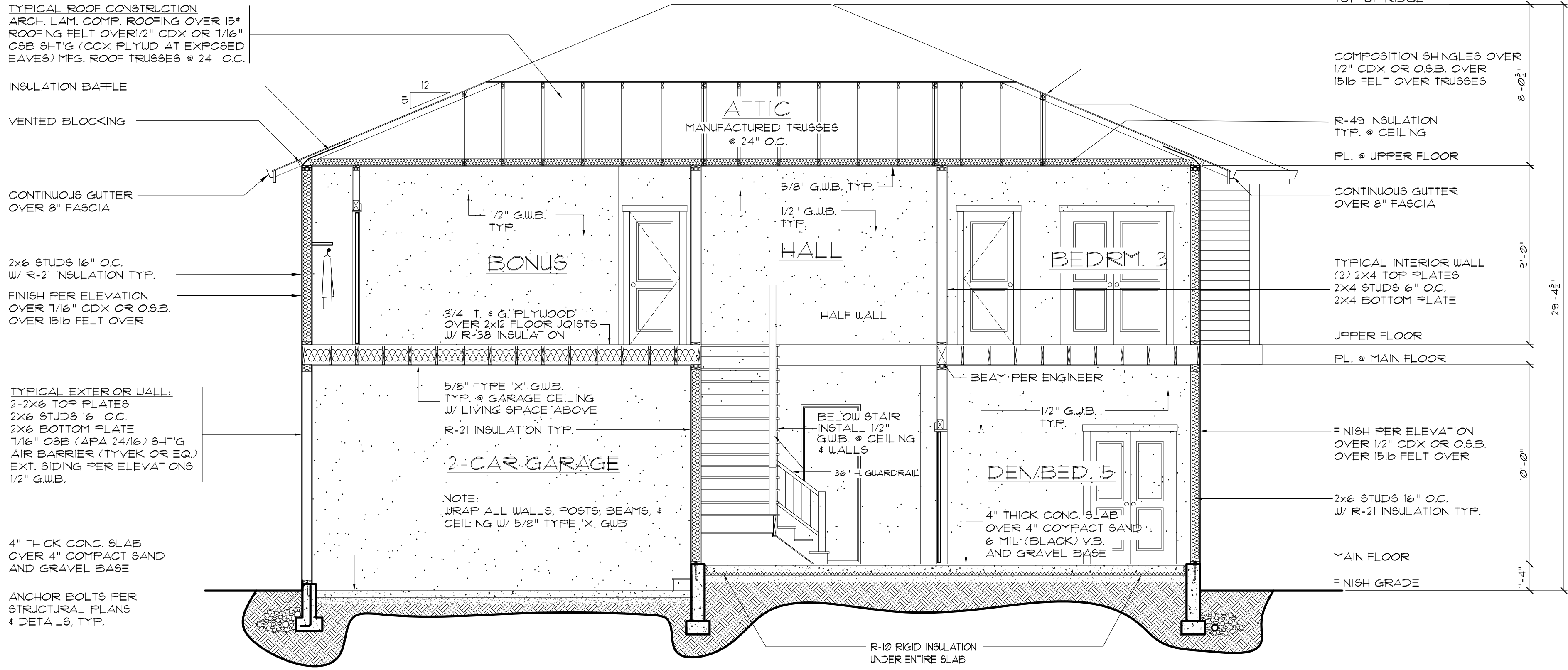
BUILDING CROSS-SECTION 'A'
