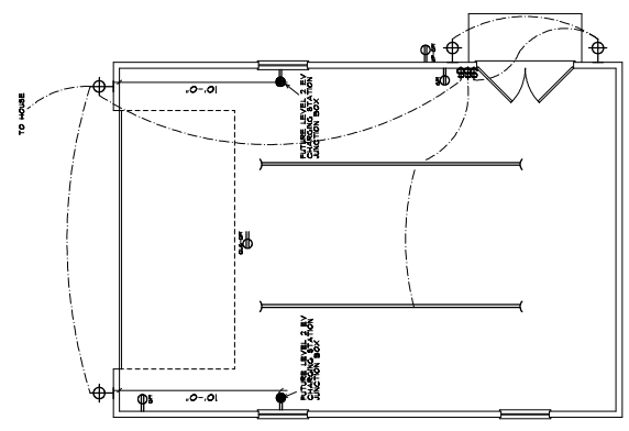
DET. GARAGE ELECTRICAL PLAN SCALE 1/4" = 1'-0"
