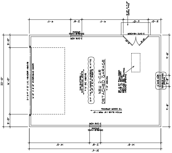
DET. GARAGE CONSTRUCTION PLAN SCALE 1/4" = 1'-0"
