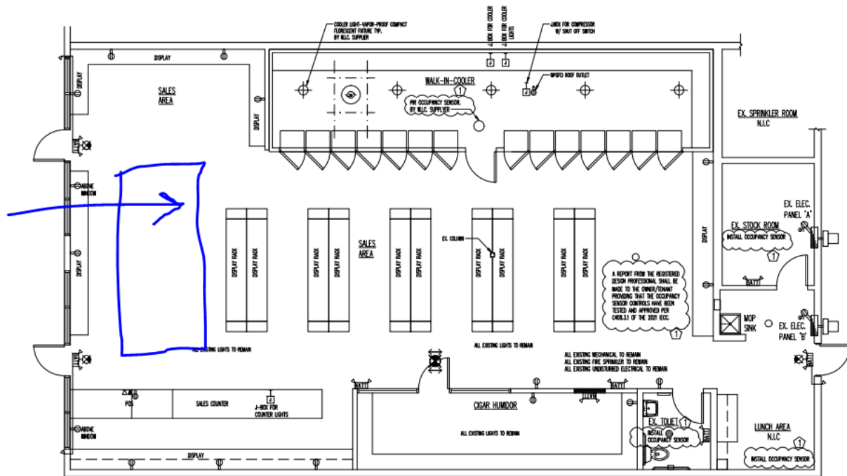
ELECTRICAL PLAN
