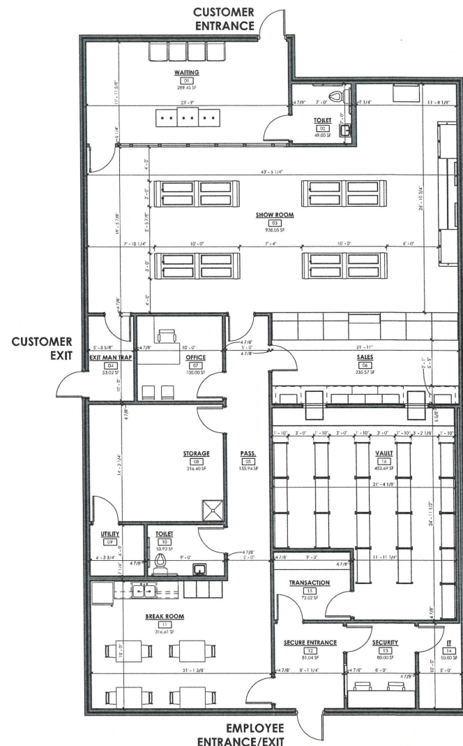
01 FLOOR PLAN 1/4" = 1'-0"
