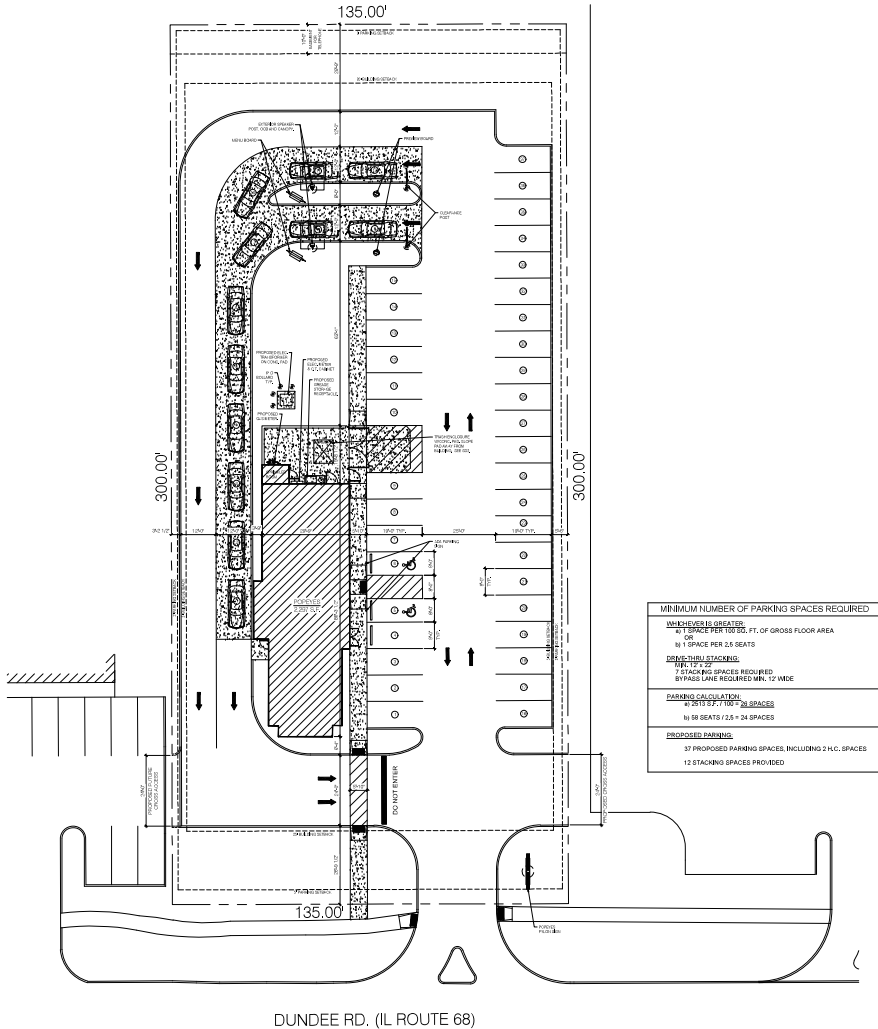
ARCHITECTURAL SITE PLAN 1"=30'-0"
