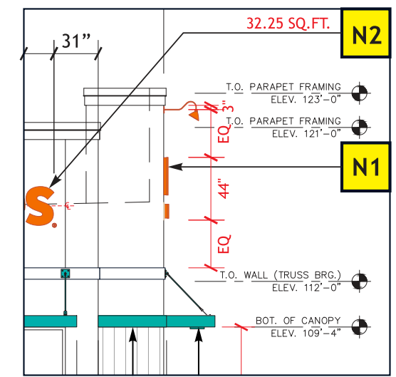
GOOSENECK LIGHT PLACEMENT SIDE ELEVATION VIEW
