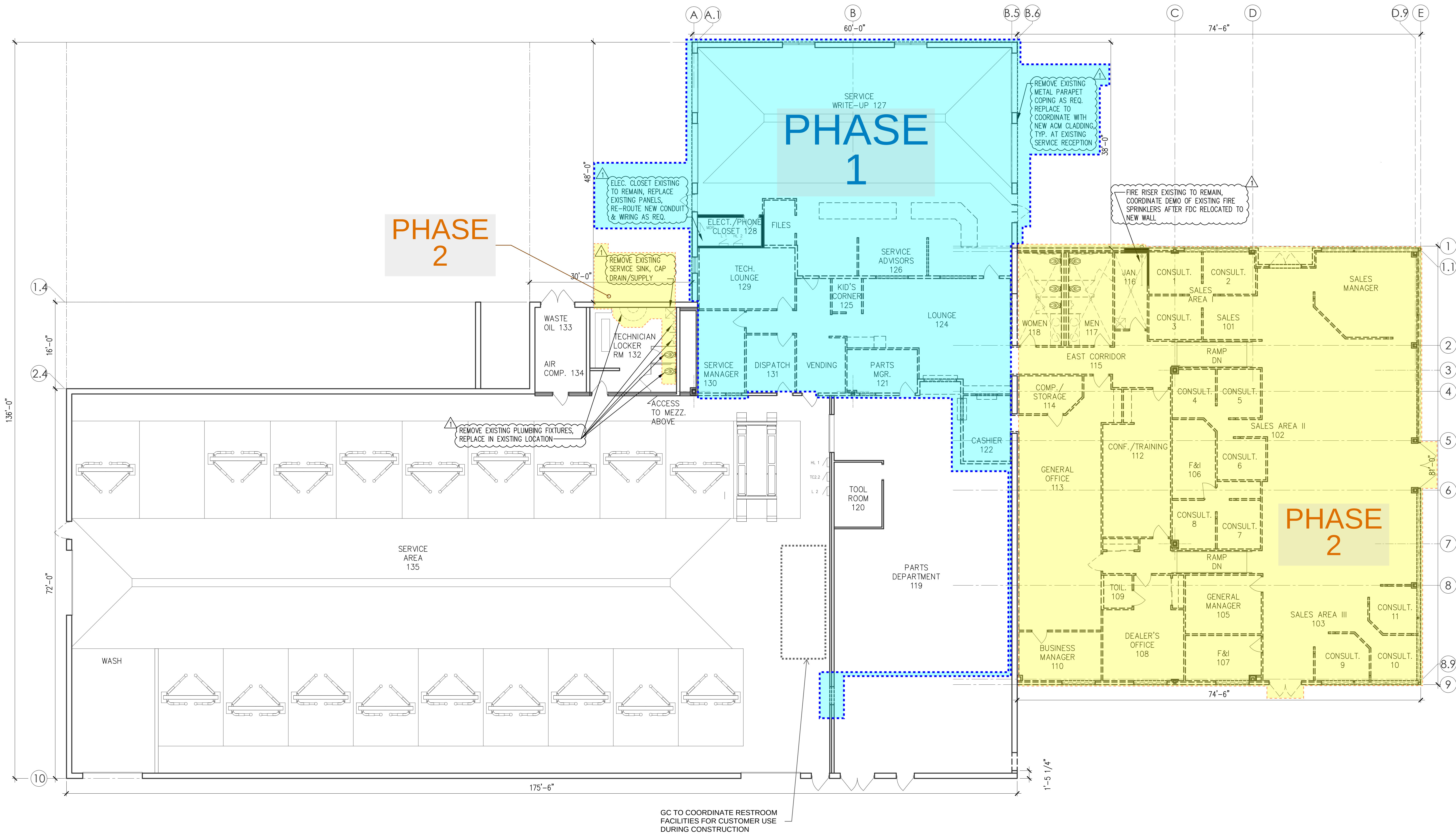
DEMOLITION PLAN - LEVEL 1 SCALE: 1/8"
