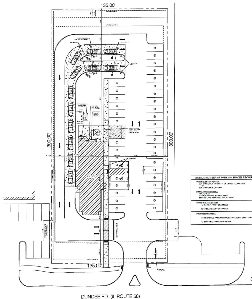
3 ARCHITECTURAL SITE PLAN SD1 1"=20'-0"
