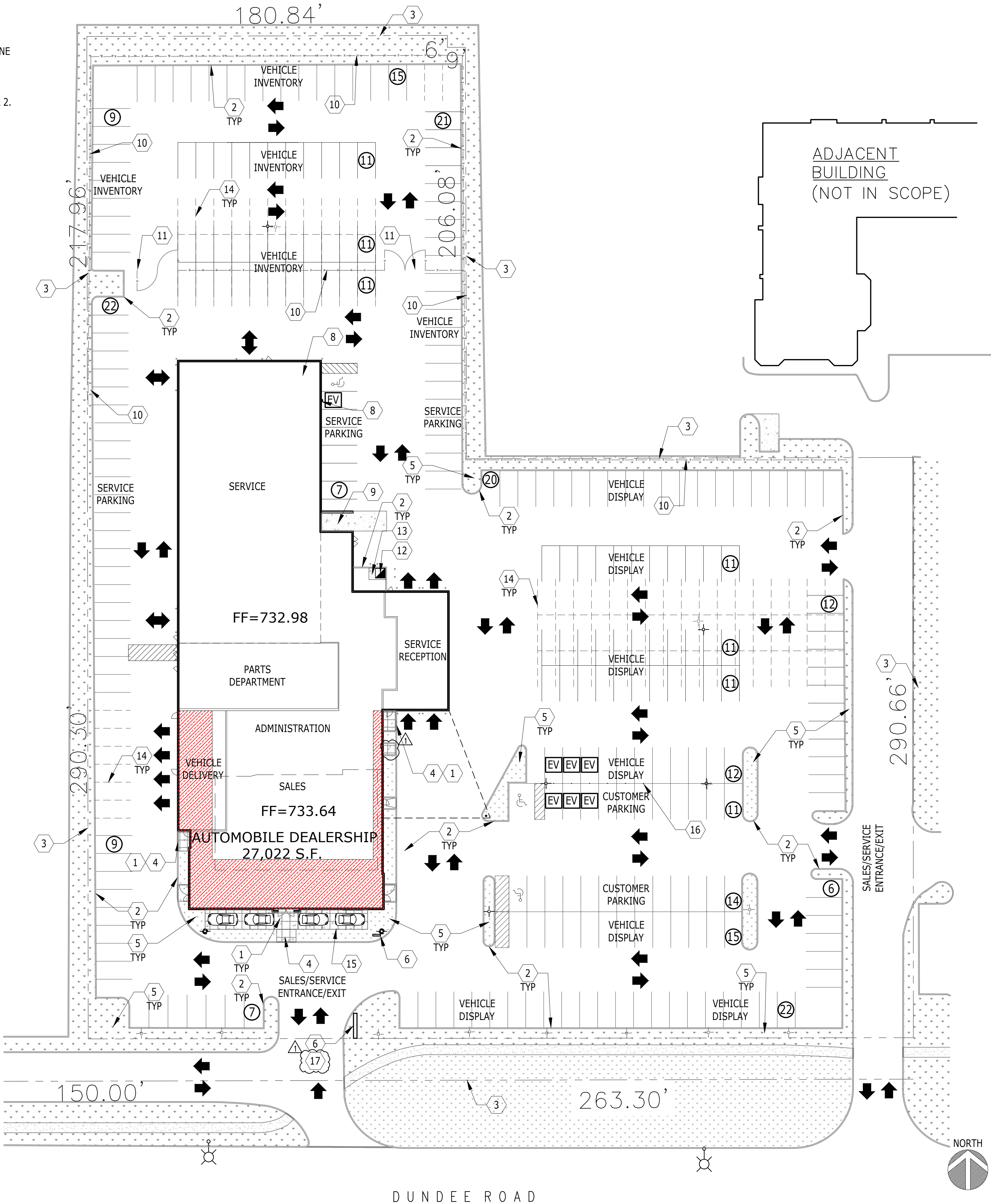
ARCHITECTURAL SITE PLAN SCALE: 1" = 30'-0"
