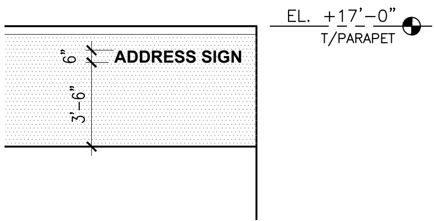
ADDRESS SIGNAGE DETAIL
