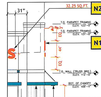
GOOSENECK LIGHT PLACEMENT SIDE ELEVATION VIEW
