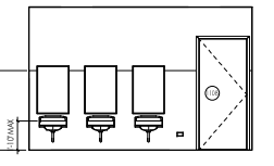
6 TODDLER 112 - SOUTH 1/4" = 1'-0"
