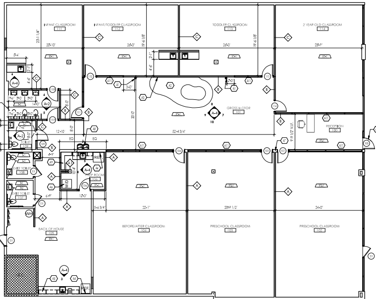
1 CONSTRUCTION PLAN 1/8" = 1'-0"
