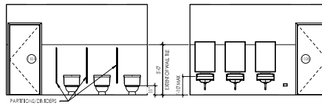
5 TODDLER 112 - NORTH 1/4" = 1'-0"
