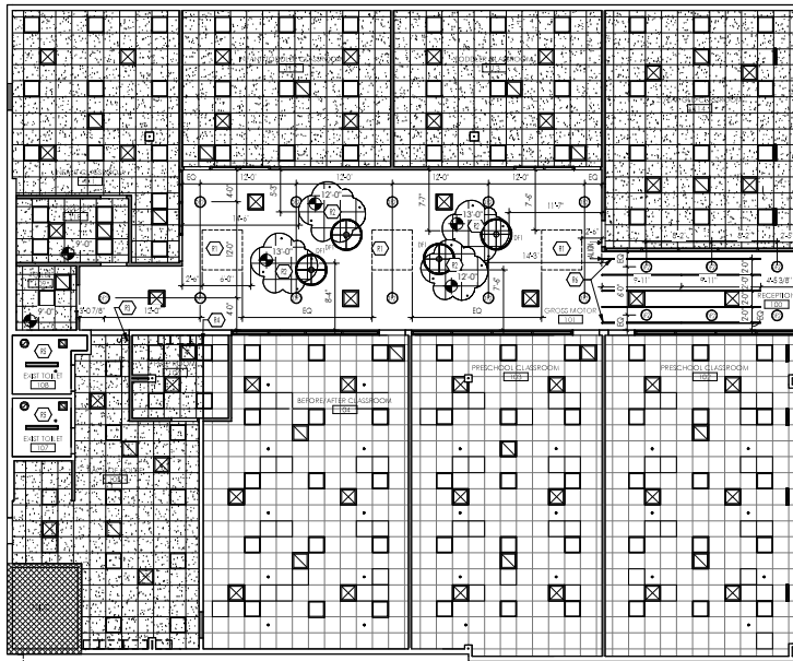
4 REFLECTED CEILING PLAN 1/8" = 1'-0"
