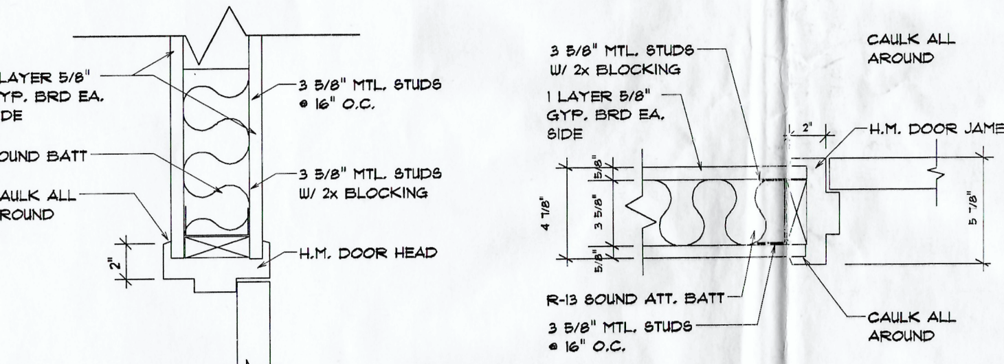
HM. DOOR JAMBS & HEAD DETAILS SCALE: NTS
