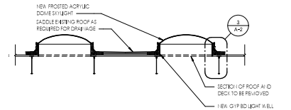
2 SKYLIGHT SECTION 1/4" = 1'-0"
