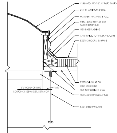
3 SKYLIGHT DETAIL 1 1/2" = 1'-0"
