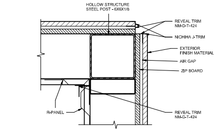
7 CORNER DETAIL 3" = 1'-0"
