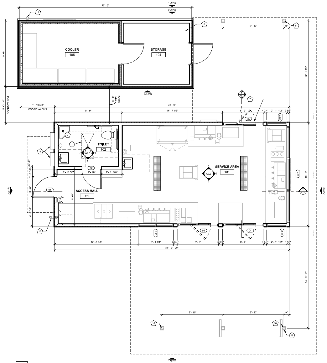
1 FLOOR PLAN
