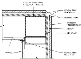
7 CORNER DETAIL 3/8" = 1'-0"
