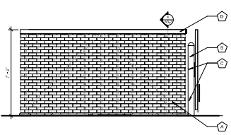
3 DUMPSTER ELEVATION - LEFT 3/8" = 1'-0"
