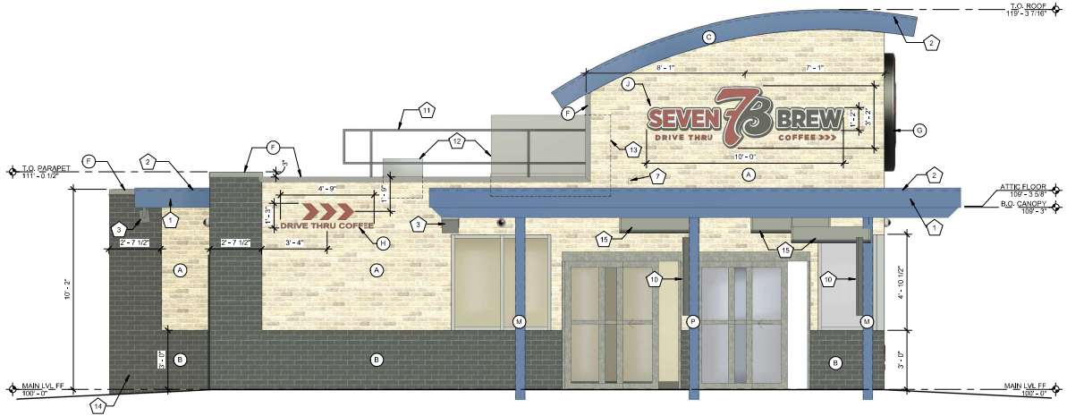
1 EXTERIOR ELEVATION - RIGHT 3/8" = 1'-0"
