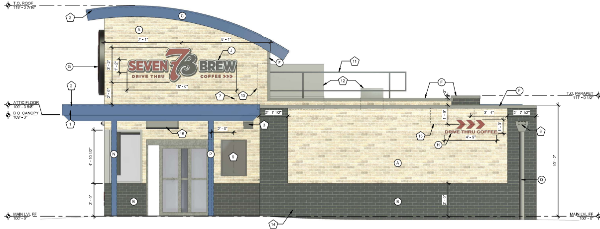
2 EXTERIOR ELEVATION - LEFT W/ COOLER 3/8" = 1'-0"
