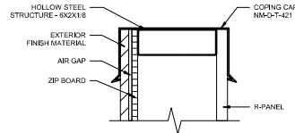
6 TOP COPING DETAIL 3" = 1'-0"
