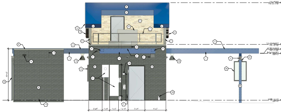
1 EXTERIOR ELEVATION - BACK 3/8" = 1'-0"
