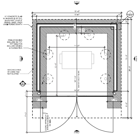
1 DUMPSTER FLOOR PLAN 3/8" = 1'-0"
