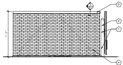
3 DUMPSTER ELEVATION - LEFT 3/8" = 1'-0"
