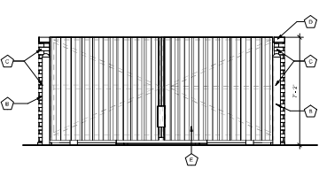
2 DUMPSTER ELEVATION - FRONT 3/8" = 1'-0"
