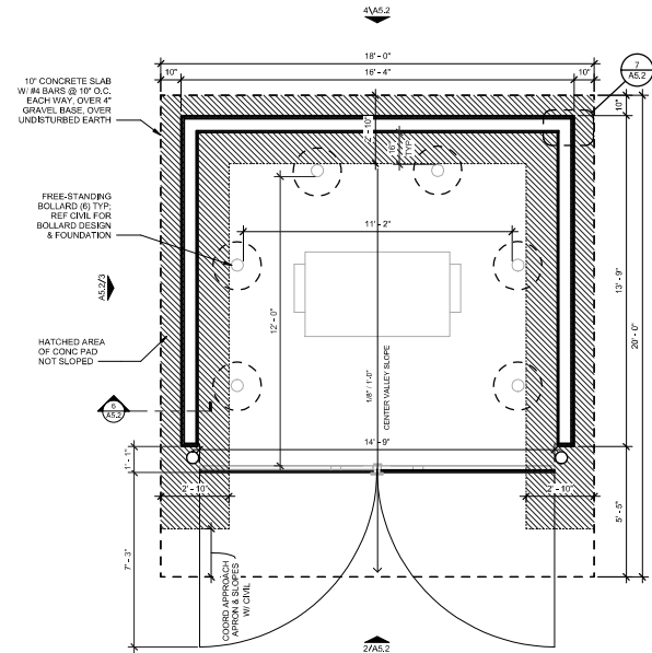
1 DUMPSTER FLOOR PLAN 3/8" = 1'-0"
